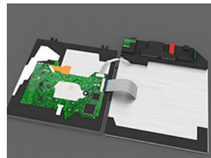
Step 8: Place DVD drive to the side
