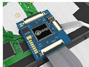
Step 11: Connect drive cable to Wiikey
