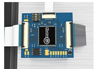
Step 13: Connect the SD card reader
