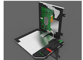
Step 7: Lift the DVD drive
